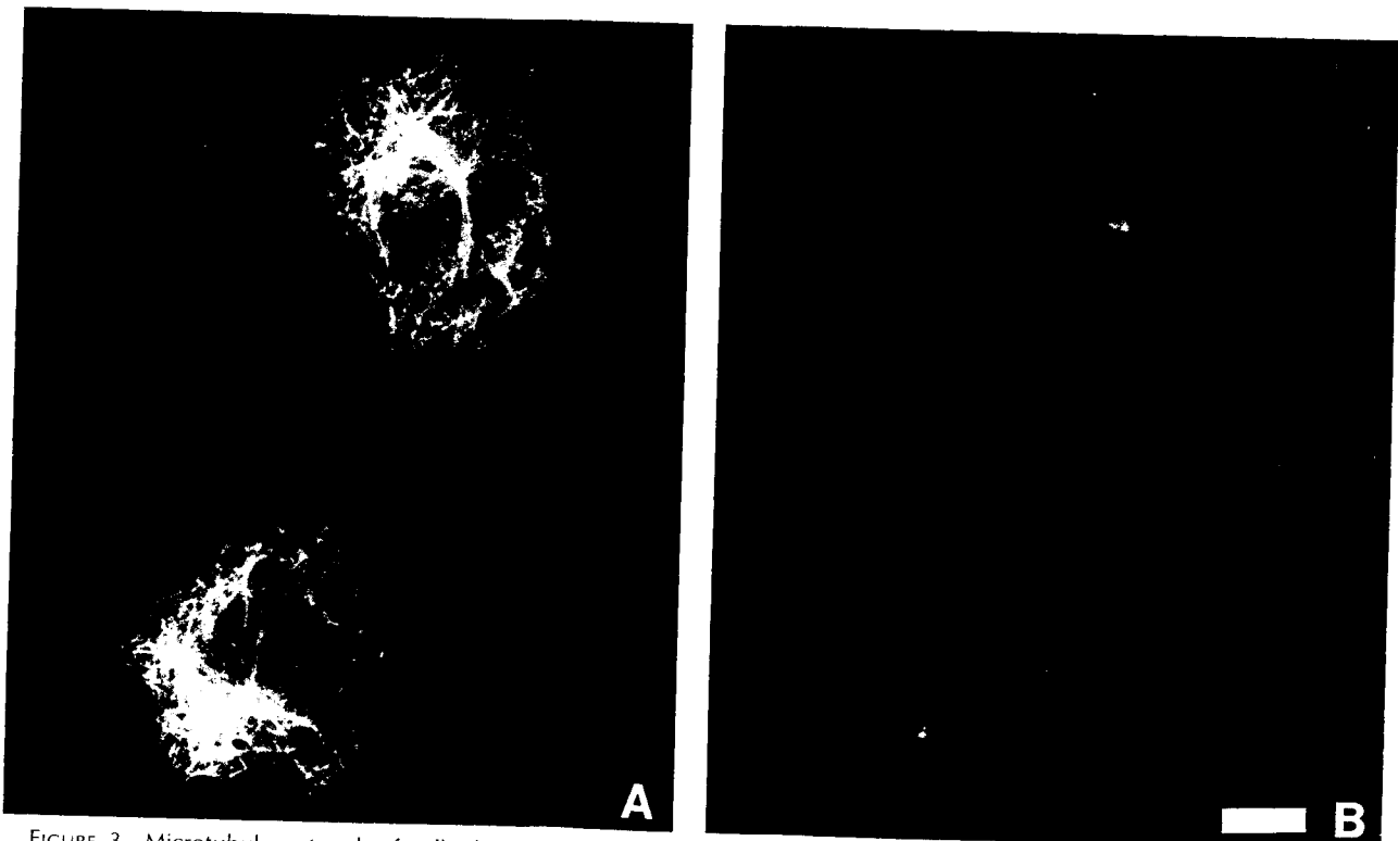
FIGURE 3 Microtubule network of cells that have been incubated in cytochalasin B and nocodazole for 1.5 h and further incubated for 18 h in normal medium. Fluorescence microscopy. (A) Microtubule staining; (B) centrosome staining of the same cells as shown in A. Bar, 10 \mu m. \times 1,000.
