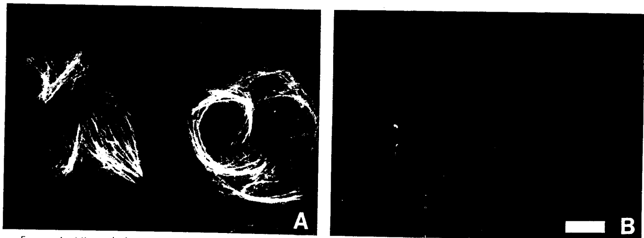
FIGURE 4 Microtubule pattern of nonconfluent cytoplasts prepared using cytochalasin B and nocodazole and further incubated in 5 \mu M taxol for 18 h after enucleation. Fluorescence microscopy. (A) Microtubule staining; (B) centrosome staining of the same cytoplasts as in A. The cytoplast on the right has no centrosome. Bar, 10 \mu m. \times 1,000.
