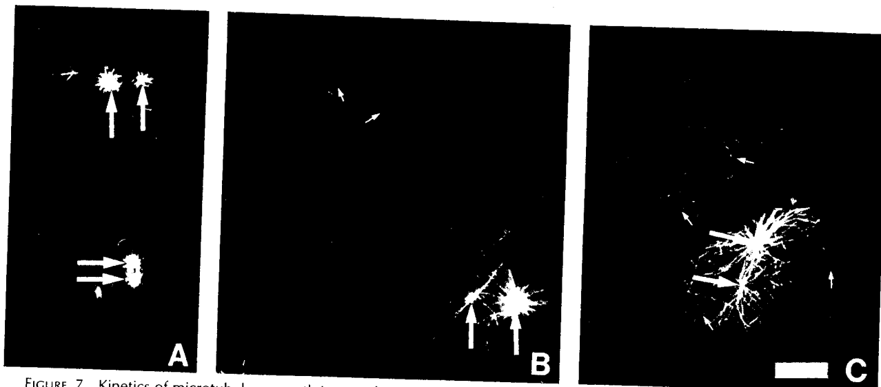
FIGURE 7 Kinetics of microtubule regrowth in cytoplasts with and without centrosomes. Cells were enucleated in the presence of cytochalasin B and nocodazole and allowed to recover from enucleation for 1 h in 10 \mu\text{g}/\text{ml} nocodazole without cytochalasin B. The cytoplasts were fixed and stained at the indicated time after transfer to regular medium. Microtubules are visualized; centrosome staining was done but not shown. (A) 3 min after nocodazole removal. Two cytoplasts are shown. The centrosome is split in both (arrows). Very short microtubules scattered in the cytoplast are also visible (mainly in the cell at the top of the figure). (B) 5 min after the nocodazole removal. Cell at the bottom of the figure has a split centrosome (large arrows). Cell at the top has no centrosome. Short free microtubules are visible (small arrows). (C) 7 min after nocodazole removal. Cell at the bottom has a split centrosome (large arrows). Cell at the top has no centrosome. Centrosome microtubules have almost reached their full length. Some free microtubules could be seen in the cytoplasts with and without centrosomes (small arrows). Bar, 10 \mu\text{m} . \times 1,000 .
