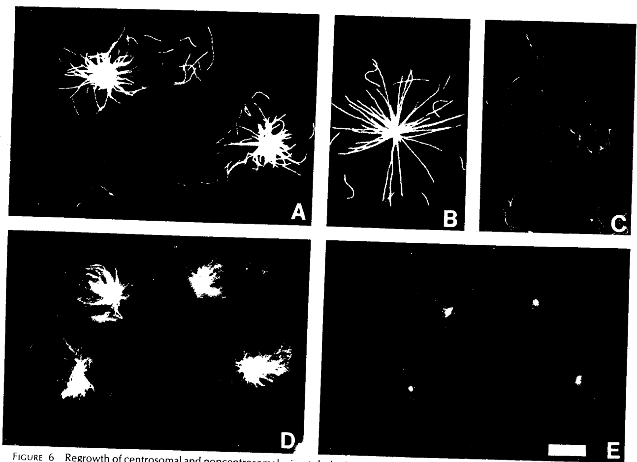
FIGURE 6 Regrowth of centrosomal and noncentrosomal microtubules in 0.1 \mu\text{g/ml} nocodazole. In A–C, cytoplasts were prepared from confluent cells in the presence of cytochalasin B and nocodazole (10 \mu\text{g/ml} ). After a 2-h incubation in 0.1 \mu\text{g/ml} nocodazole they were stained with antibodies to tubulin and centrosomes. Only tubulin staining is shown in A–C. (A) Typical microtubule pattern. Many microtubules regrow from the centrosome. Their length is heterogeneous. Very few free microtubules are visible by the centrosome could be counted. (C) Two cytoplasts lacking a centrosome are shown. A few, randomly organized microtubules are formed. Their length is variable. (D) Cells preincubated in cytochalasin B and nocodazole (10 \mu\text{g/ml} ) for 1.5 h, further incubated for 2 h in 0.1 \mu\text{g/ml} nocodazole, and fixed. Microtubule staining: most microtubules originate from the centrosome. Because of the thickness of the nucleus, the whole cell cannot be brought to focus at the same plane. (E) Centrosome staining of the cells shown in D. Bar, 8 \mu\text{m} . \times 1,300 .
